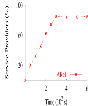
Figure 8: Discouraging free-riding
